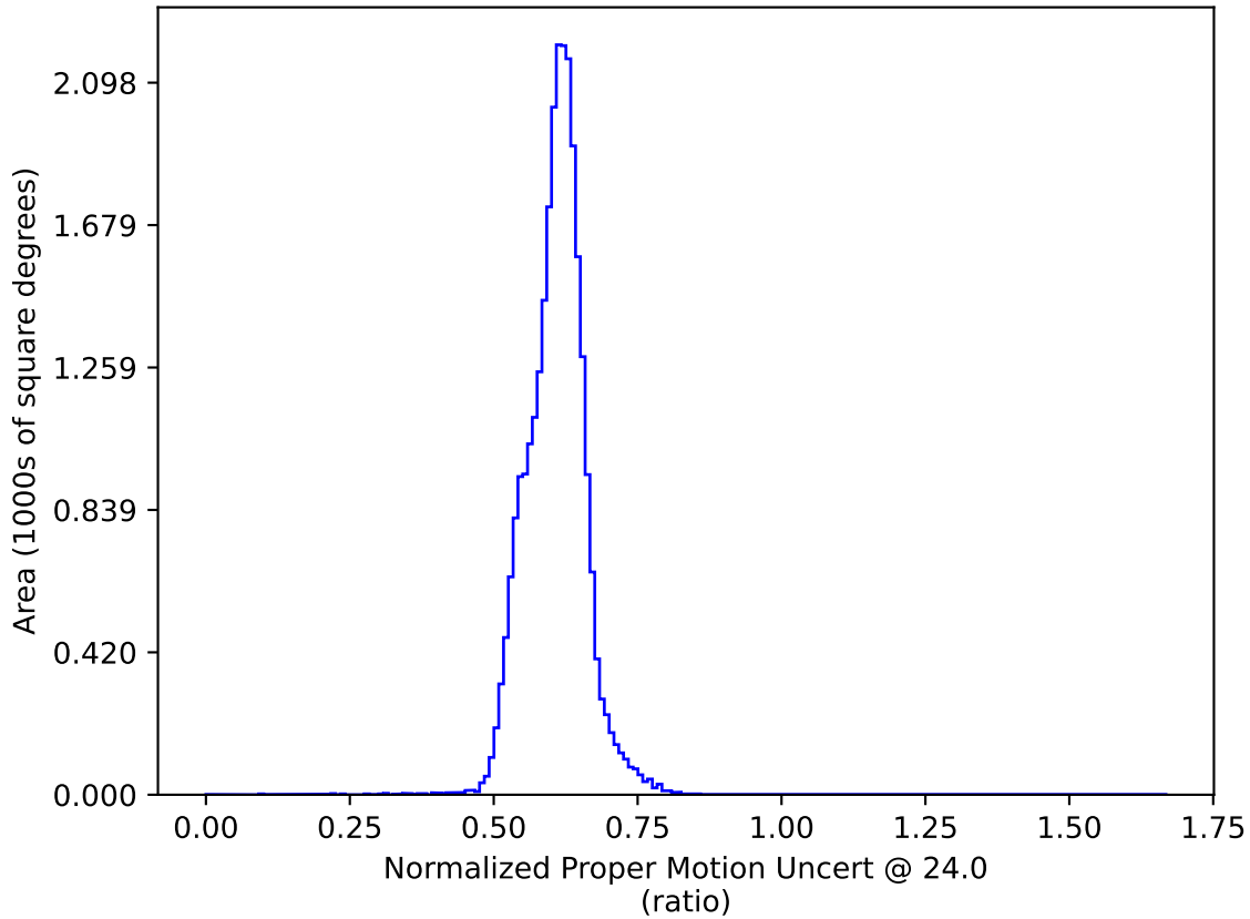
too_elab_r8_d3_ugrizy_v3.4_10yrs All sky: Normalized Proper Motion Uncert @ 24.0
