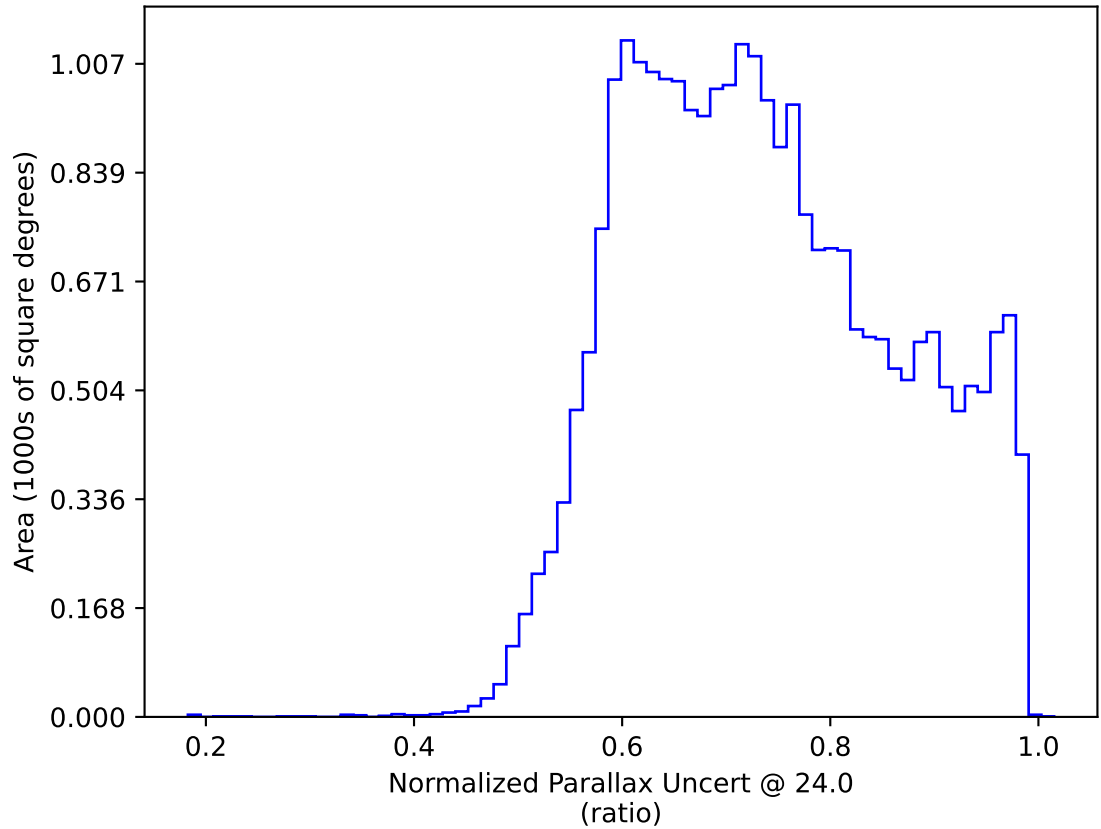
too_elab_r8_d3_ugrizy_v3.4_10yrs All sky: Normalized Parallax Uncert @ 24.0
