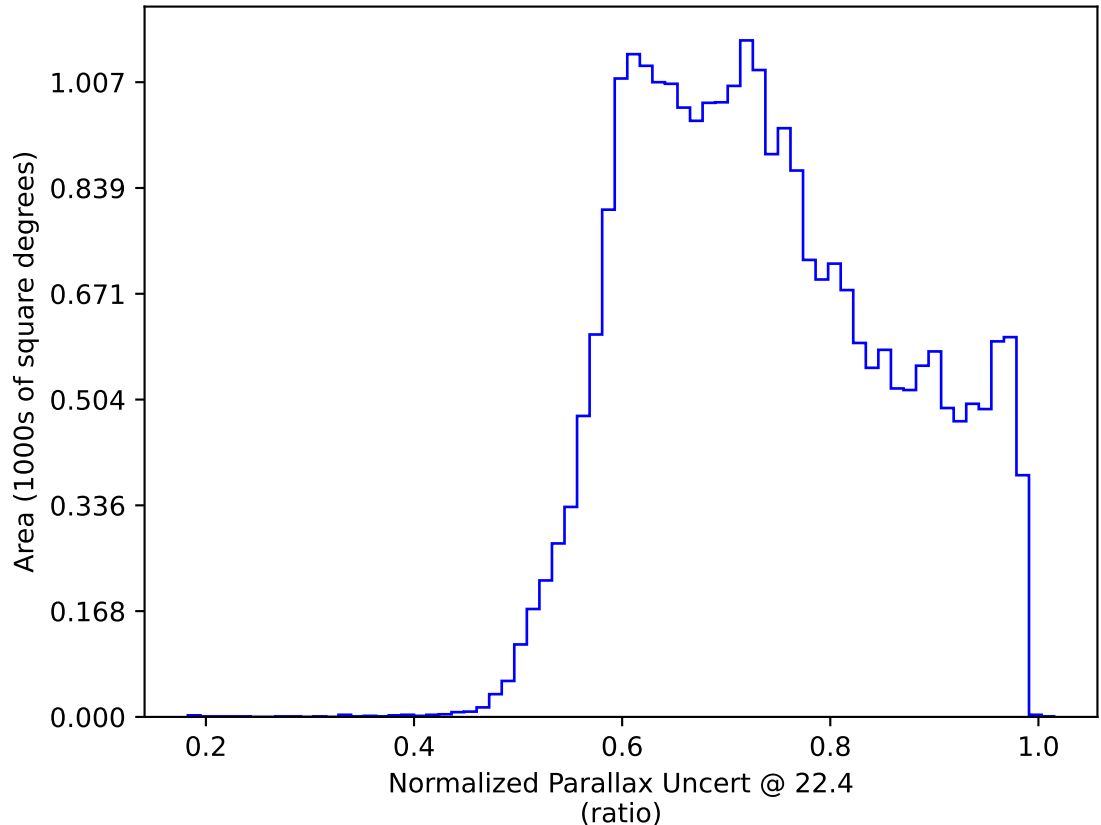
too_elab_r8_d3_ugrizy_v3.4_10yrs All sky: Normalized Parallax Uncert @ 22.4
