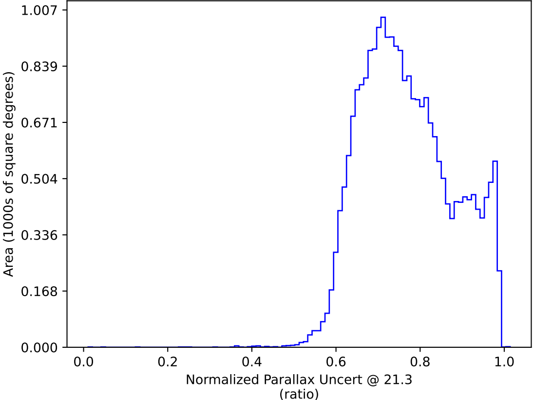
too_elab_r8_d3_ugrizy_v3.4_10yrs All sky y band only: Normalized Parallax Uncert @ 21.3
