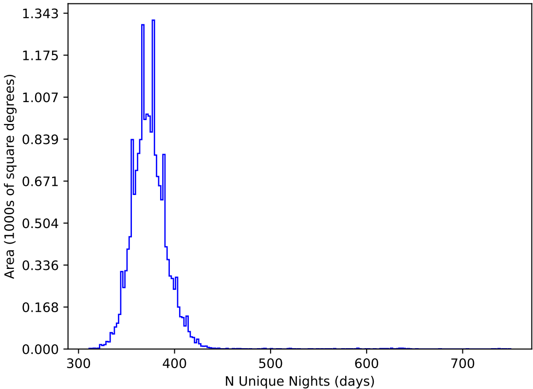
too_elab_r8_d3_ugrizy_v3.4_10yrs WFD all bands: N Unique Nights
