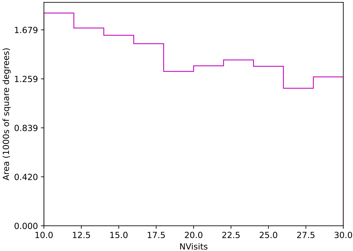
too_elab_r8_d3_ugrizy_v3.4_10yrs Yr 3-4 z band: NVisits
