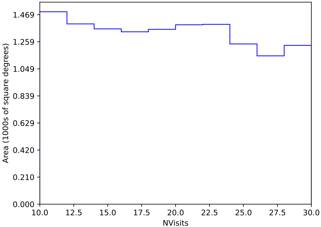
too_elab_r8_d3_ugrizy_v3.4_10yrs Yr 3-4 y band: NVisits
