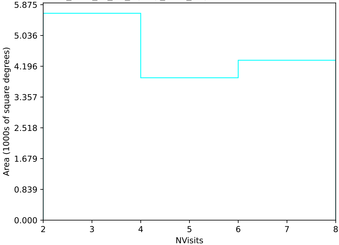
too_elab_r8_d3_ugrizy_v3.4_10yrs Yr 3-4 u band: NVisits
