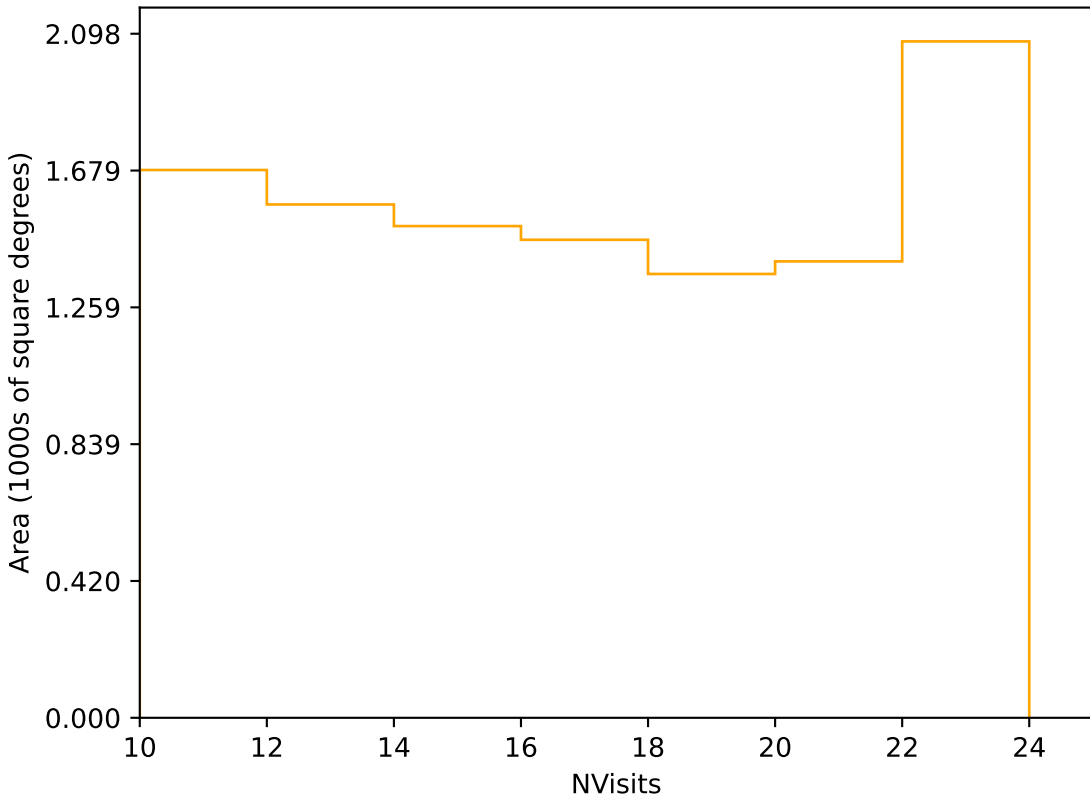
too_elab_r8_d3_ugrizy_v3.4_10yrs Yr 3-4 r band: NVisits
