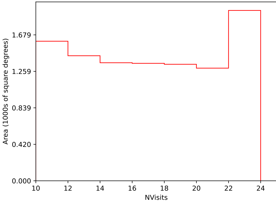
too_elab_r8_d3_ugrizy_v3.4_10yrs Yr 3-4 i band: NVisits
