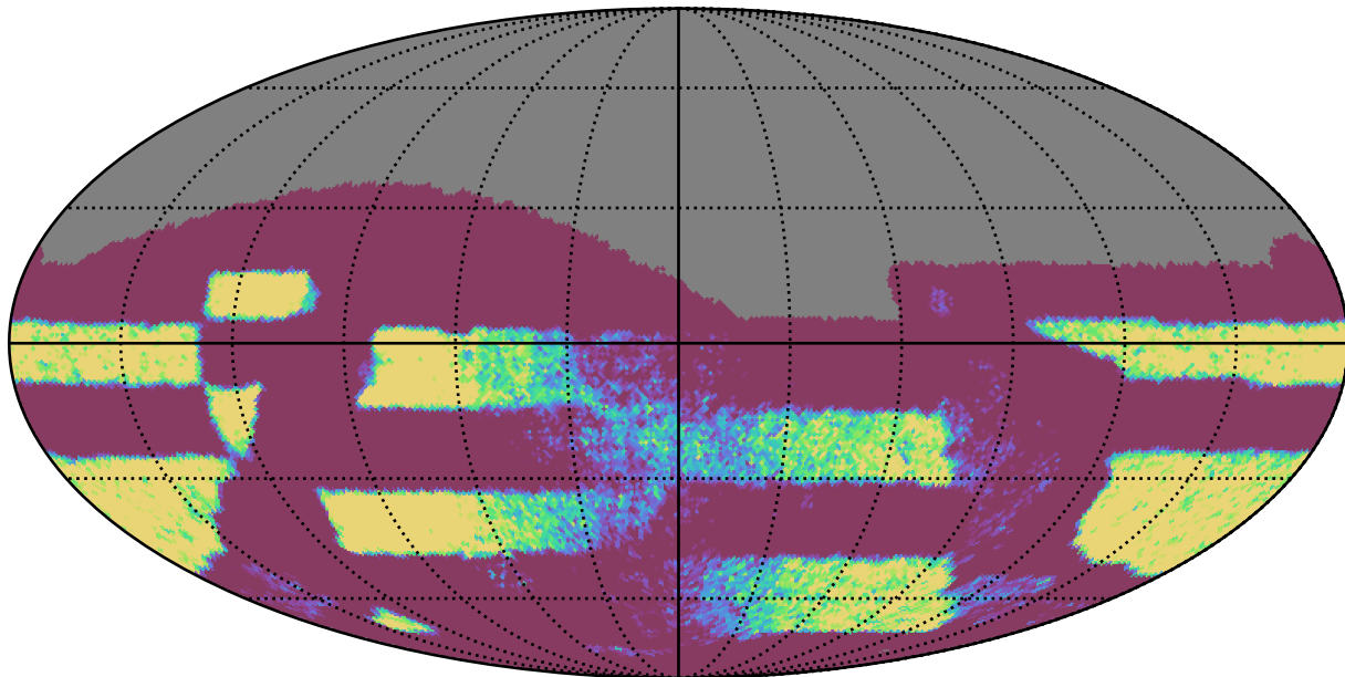
too_elab_r8_d3_ugrizy_v3.4_10yrs Yr 3-4 all bands: NVisits
