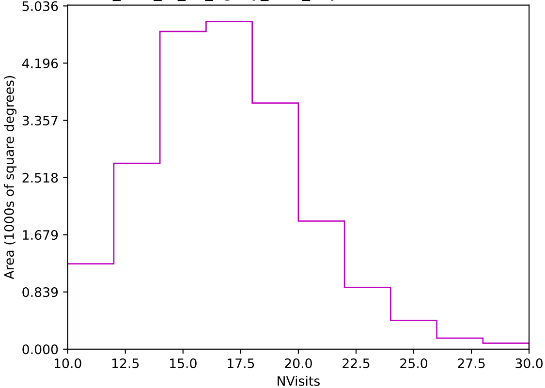
too_elab_r8_d3_ugrizy_v3.4_10yrs Yr 1 z band: NVisits
