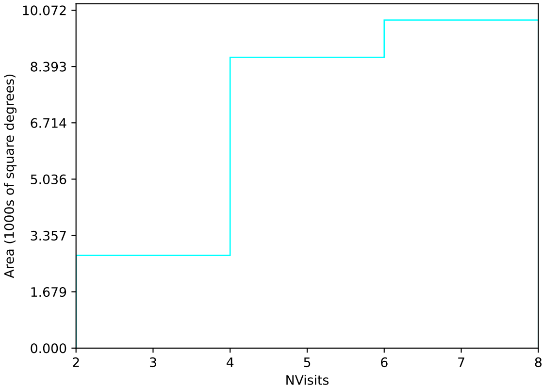
too_elab_r8_d3_ugrizy_v3.4_10yrs Yr 1 u band: NVisits
