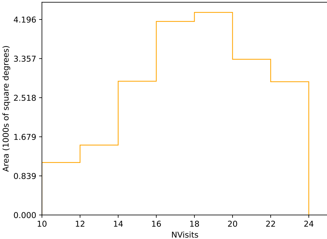
too_elab_r8_d3_ugrizy_v3.4_10yrs Yr 1 r band: NVisits
