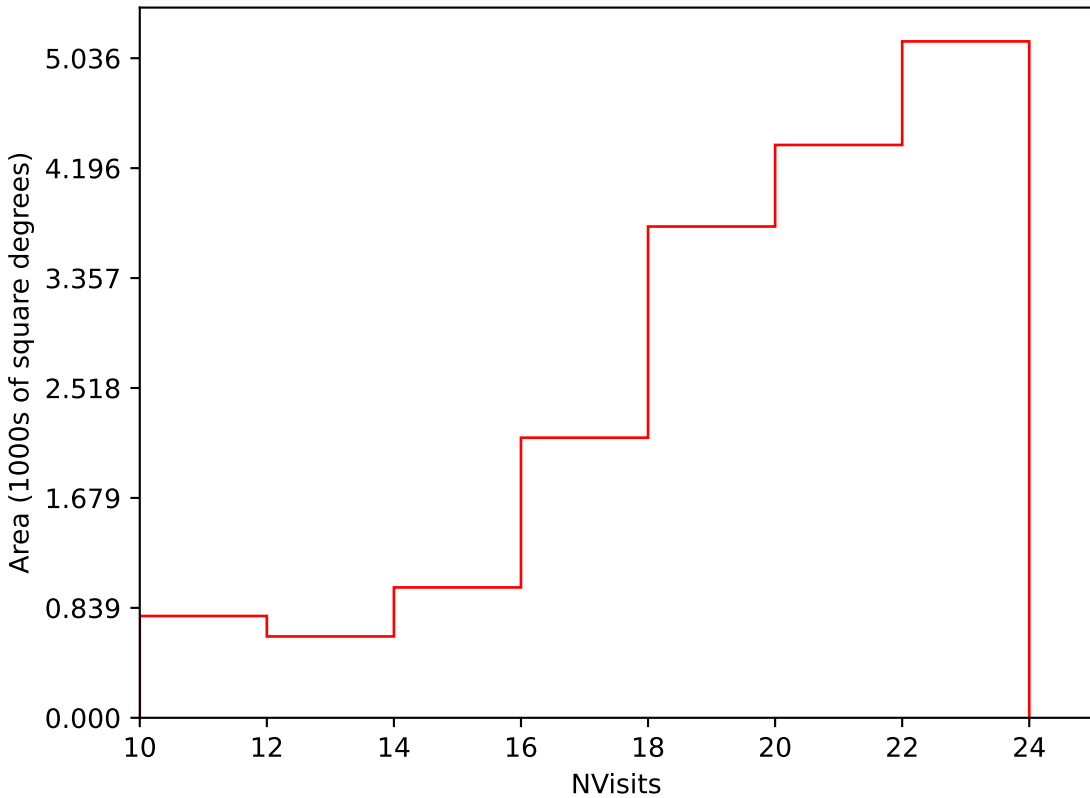
too_elab_r8_d3_ugrizy_v3.4_10yrs Yr 1 i band: NVisits
