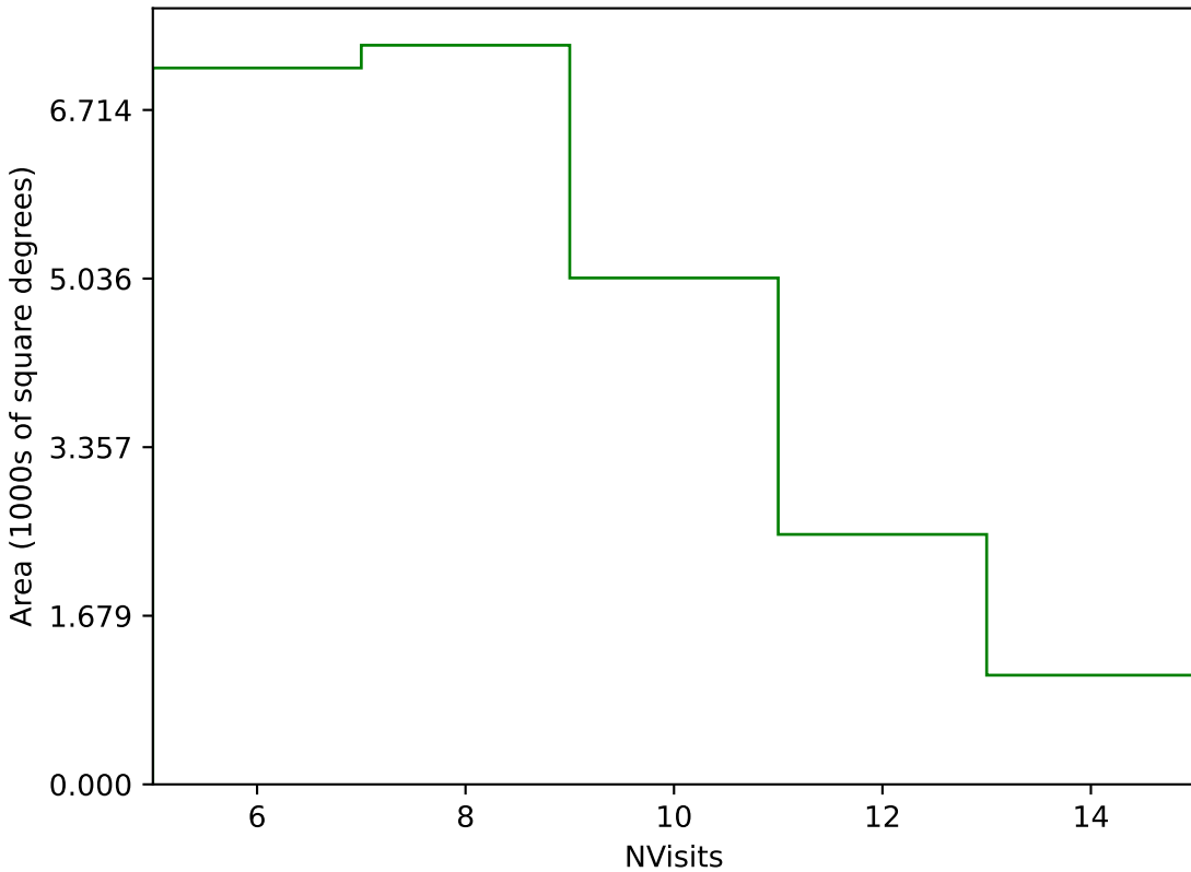
too_elab_r8_d3_ugrizy_v3.4_10yrs Yr 1 g band: NVisits
