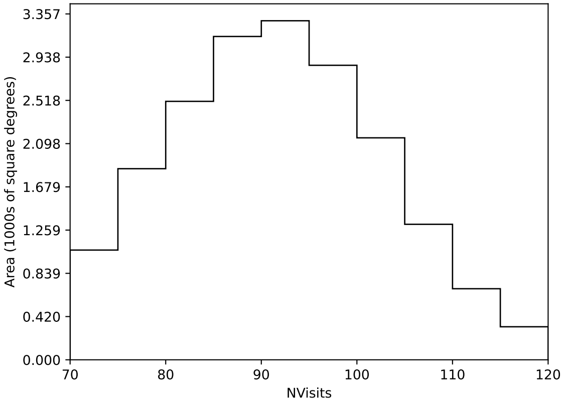
too_elab_r8_d3_ugrizy_v3.4_10yrs Yr 1 all bands: NVisits
