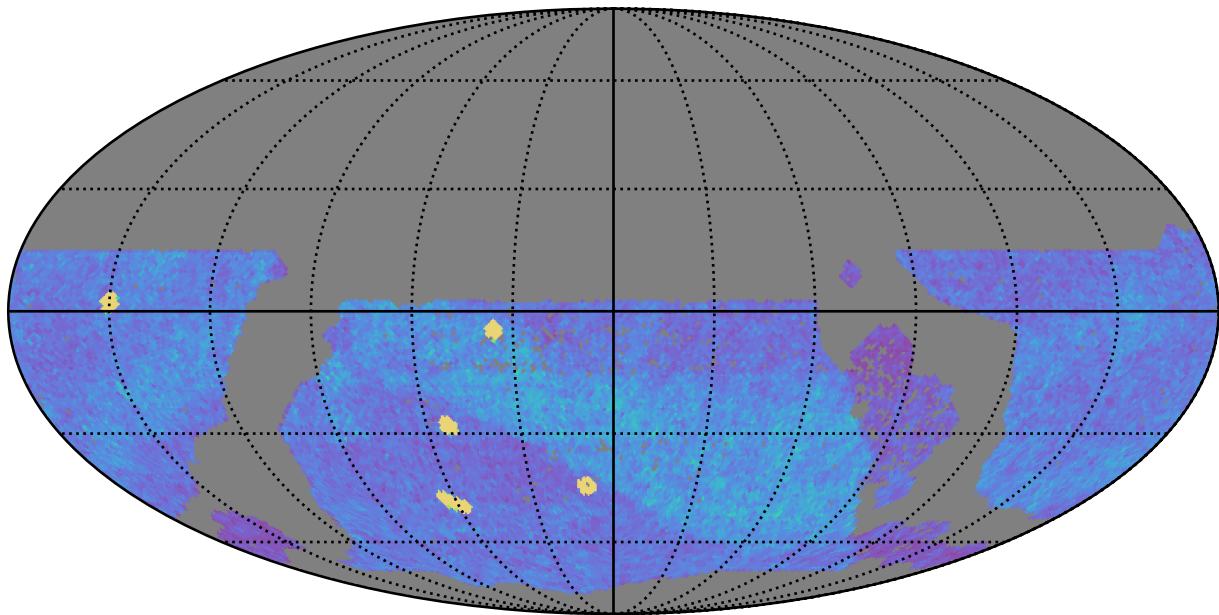
too_elab_r8_d3_ugrizy_v3.4_10yrs WFD z band: NVisits
