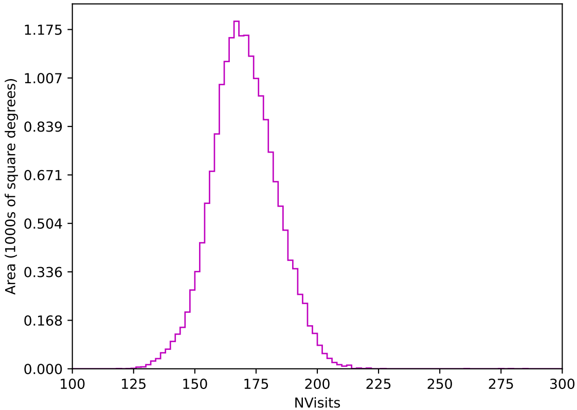
too_elab_r8_d3_ugrizy_v3.4_10yrs WFD z band: NVisits
