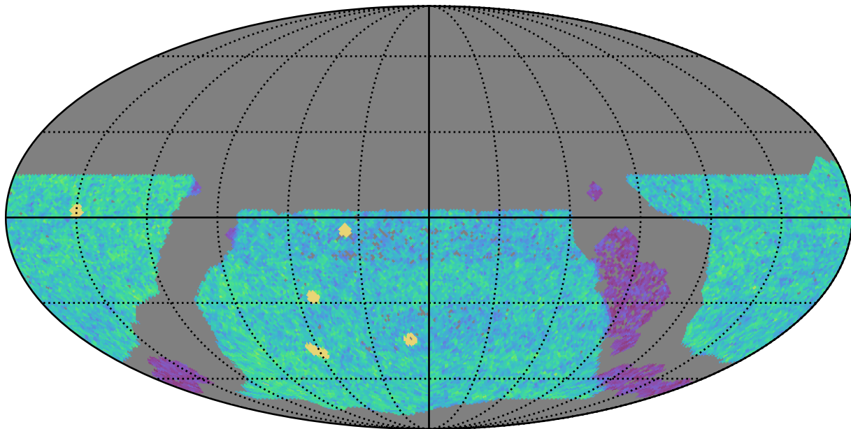
too_elab_r8_d3_ugrizy_v3.4_10yrs WFD u band: NVisits
