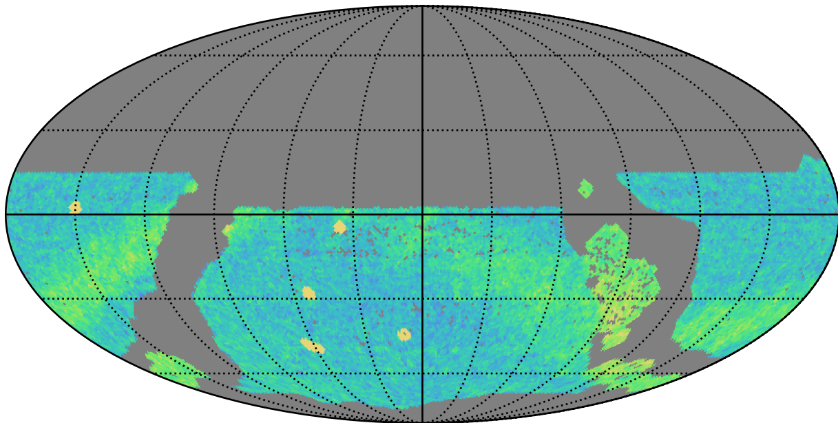
too_elab_r8_d3_ugrizy_v3.4_10yrs WFD r band: NVisits
