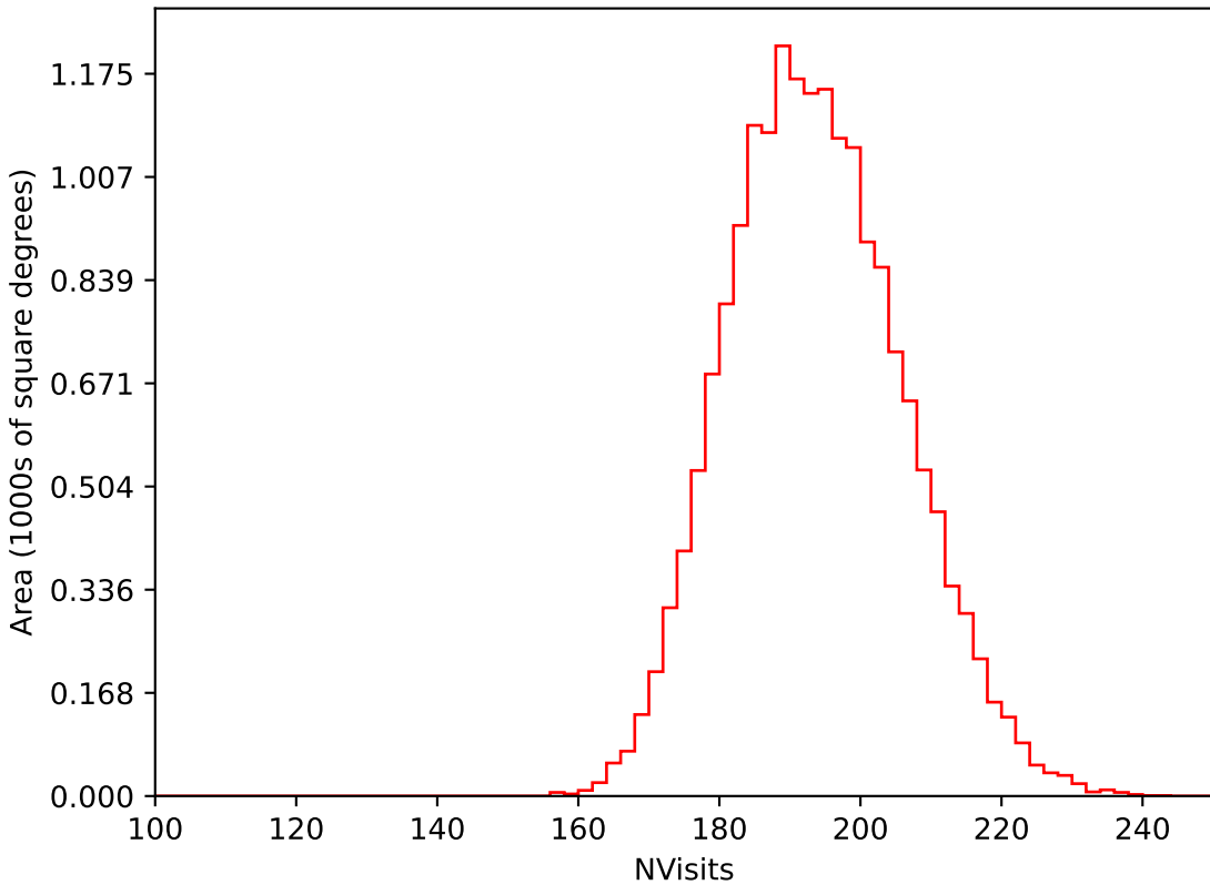
too_elab_r8_d3_ugrizy_v3.4_10yrs WFD i band: NVisits
