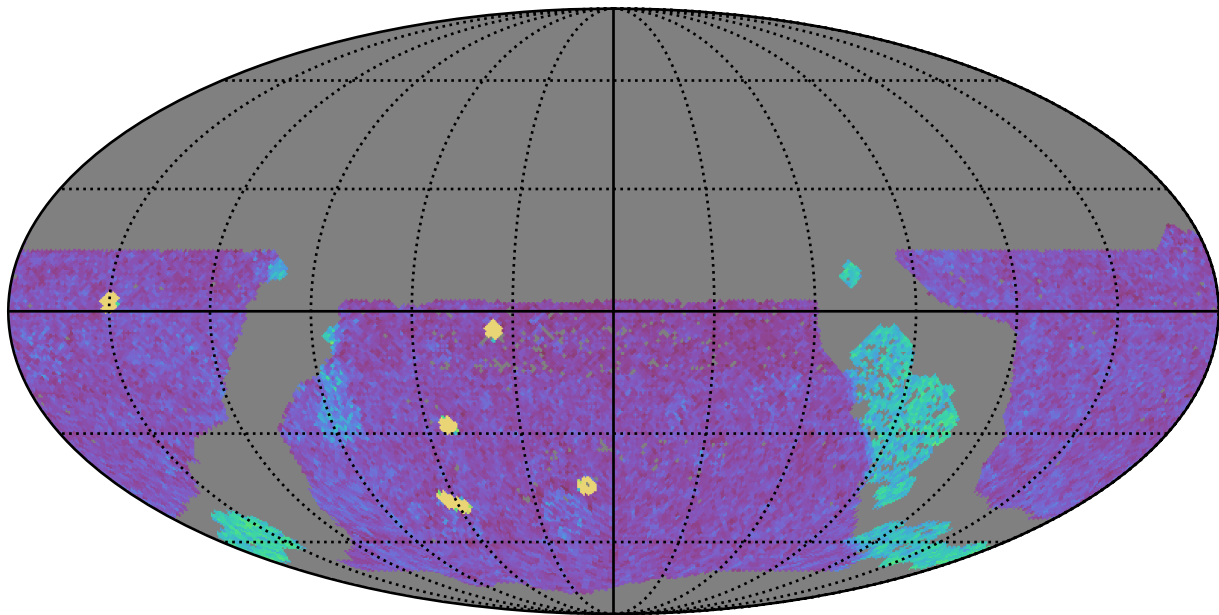
too_elab_r8_d3_ugrizy_v3.4_10yrs WFD g band: NVisits
