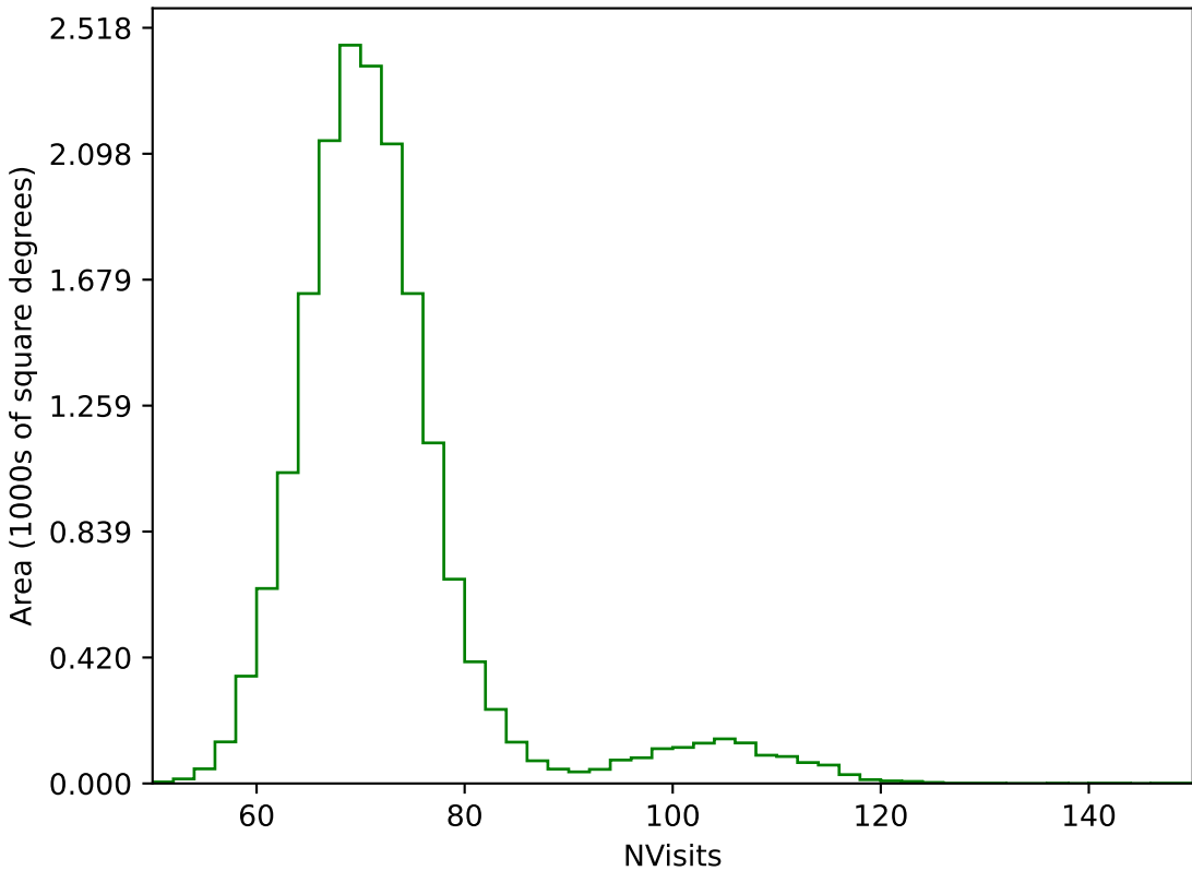
too_elab_r8_d3_ugrizy_v3.4_10yrs WFD g band: NVisits
