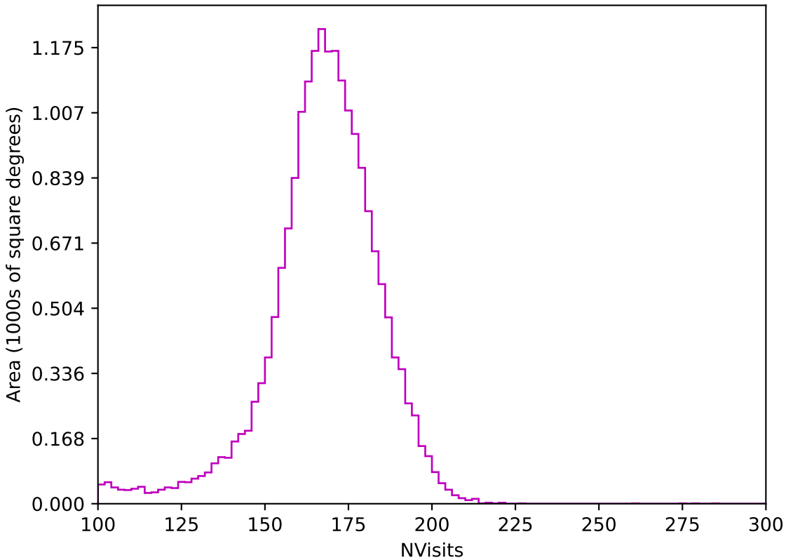
too_elab_r8_d3_ugrizy_v3.4_10yrs All sky z band: NVisits
