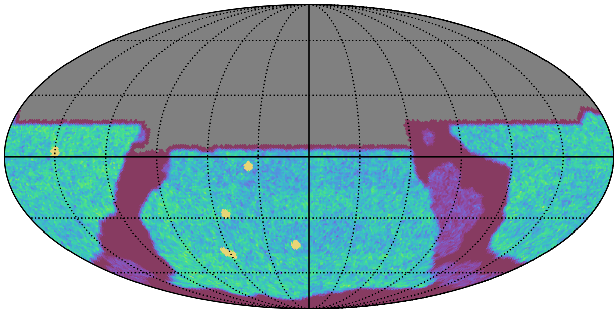
too_elab_r8_d3_ugrizy_v3.4_10yrs All sky u band: NVisits
