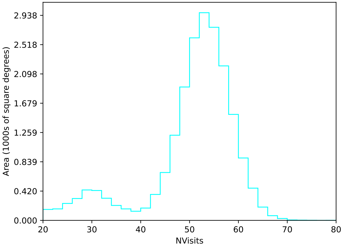
too_elab_r8_d3_ugrizy_v3.4_10yrs All sky u band: NVisits
