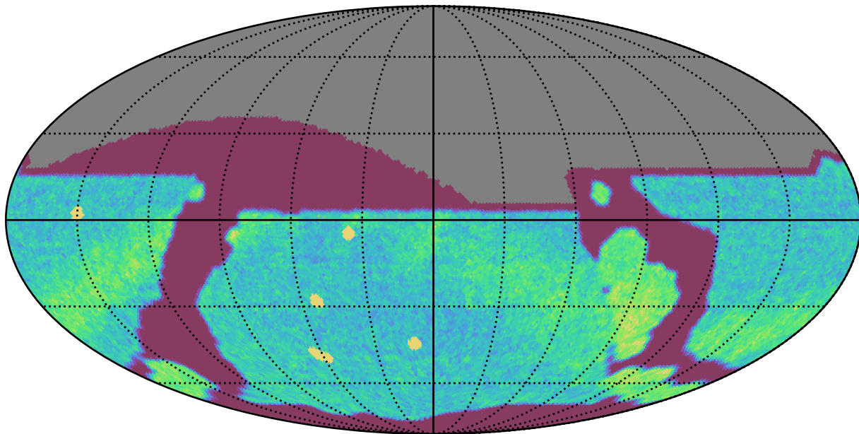
too_elab_r8_d3_ugrizy_v3.4_10yrs All sky r band: NVisits
