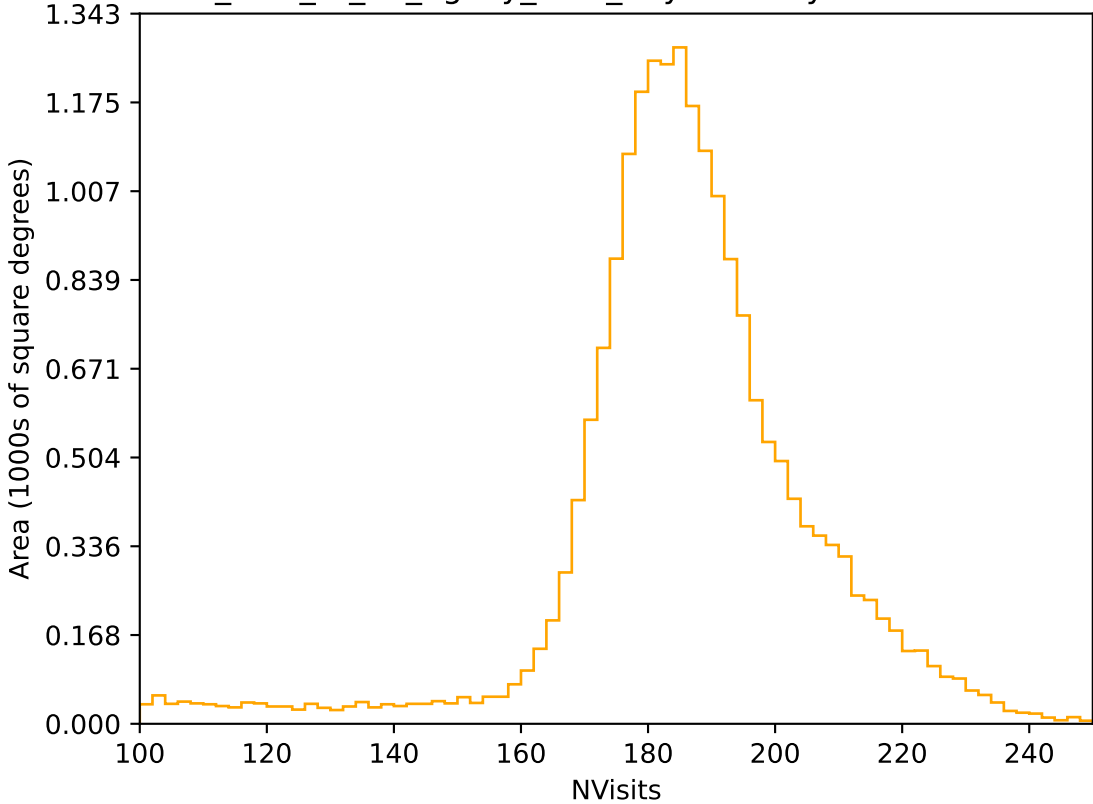
too_elab_r8_d3_ugrizy_v3.4_10yrs All sky r band: NVisits
