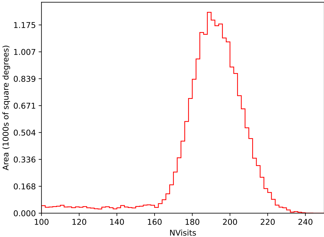
too_elab_r8_d3_ugrizy_v3.4_10yrs All sky i band: NVisits
