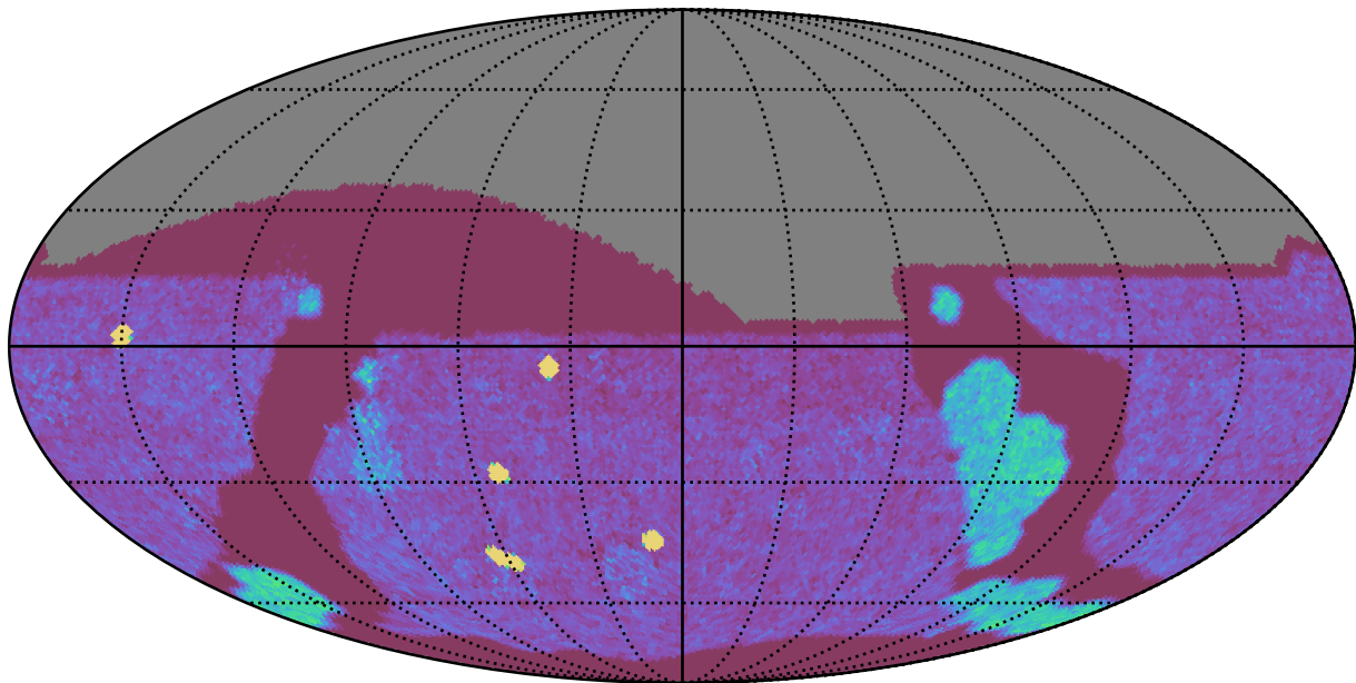
too_elab_r8_d3_ugrizy_v3.4_10yrs All sky g band: NVisits
