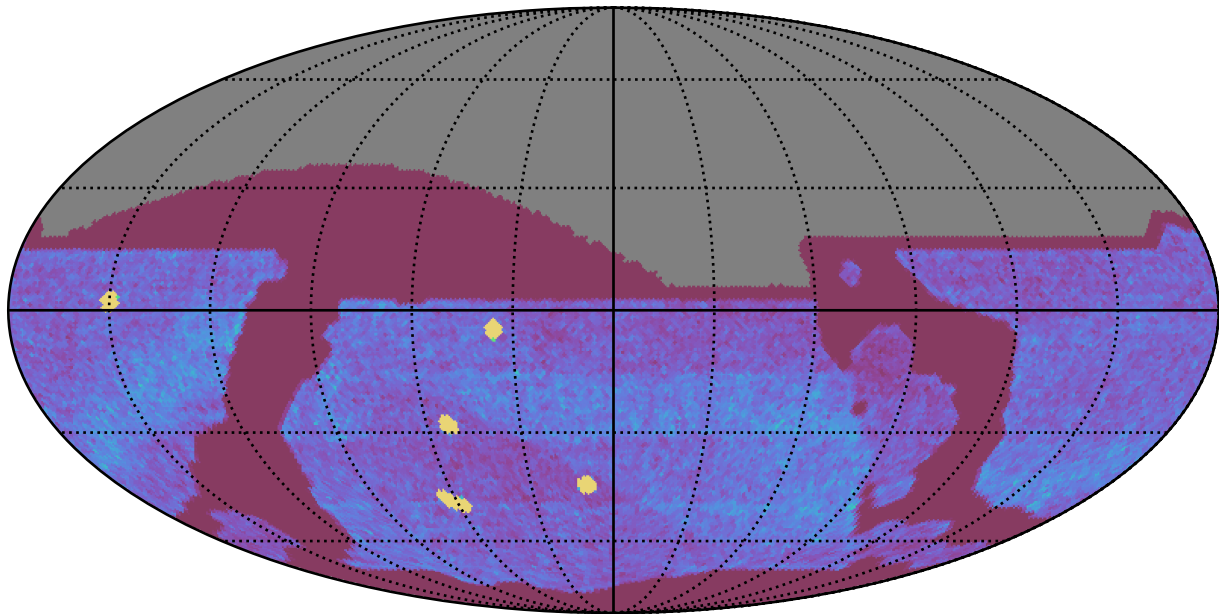
too_elab_r8_d3_ugrizy_v3.4_10yrs All sky all bands: NVisits
