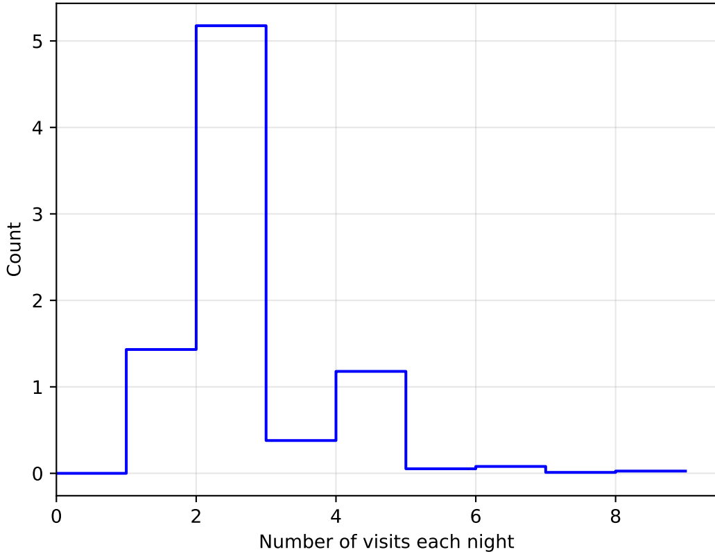
too_elab_r8_d3_ugrizy_v3.4_10yrs WFD: NVisitsPerNight
