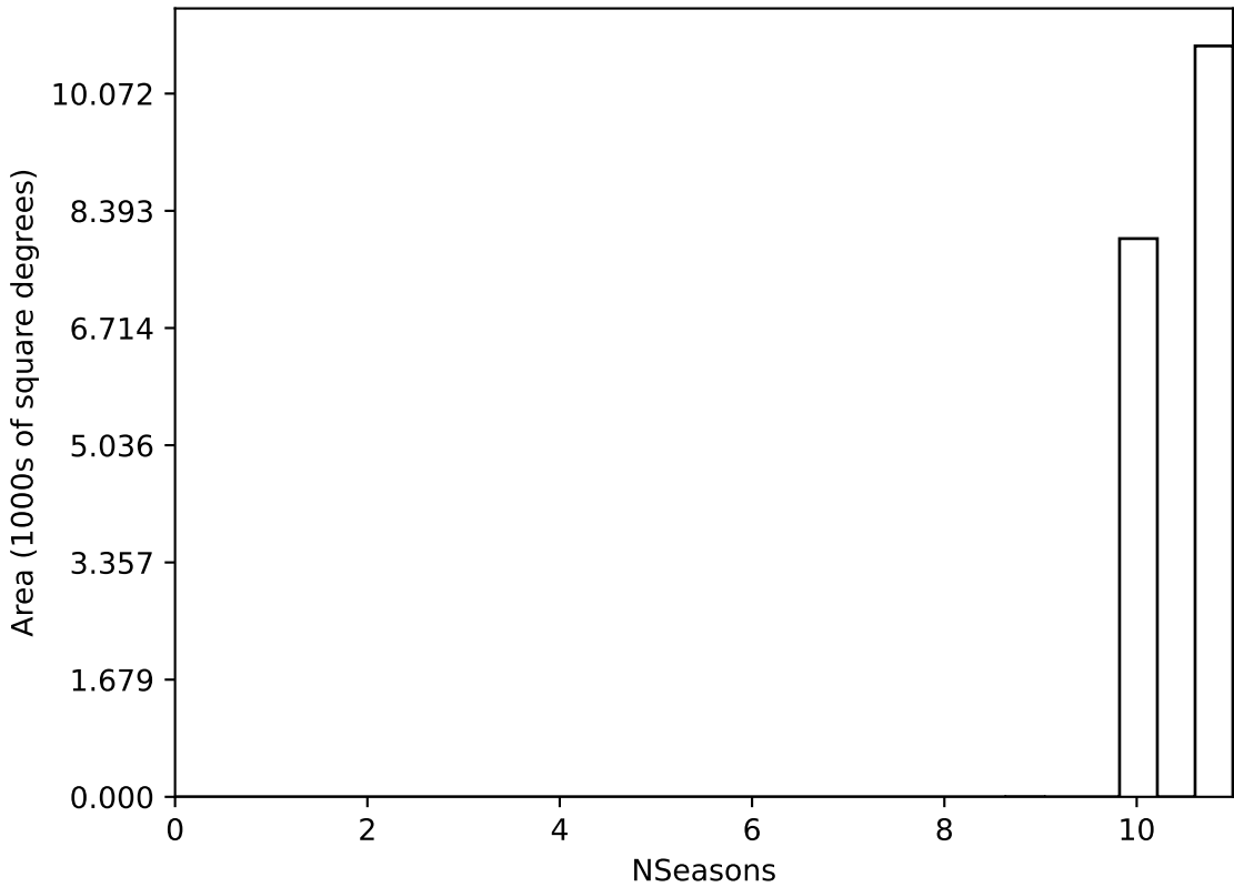
too_elab_r8_d3_ugrizy_v3.4_10yrs WFD all bands: NSeasons
