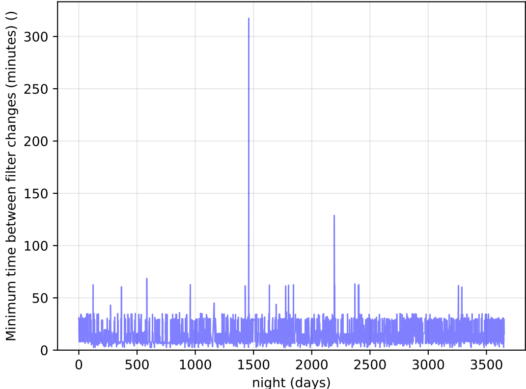
too_elab_r8_d3_ugrizy_v3.4_10yrs Per Night: Minimum time between filter changes (minutes)
