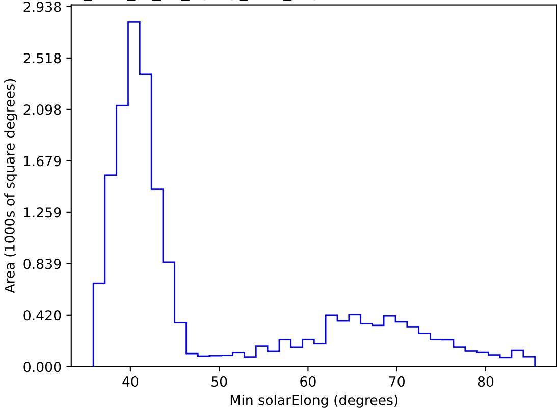
too_elab_r8_d3_ugrizy_v3.4_10yrs WFD z band: Min solarElong
