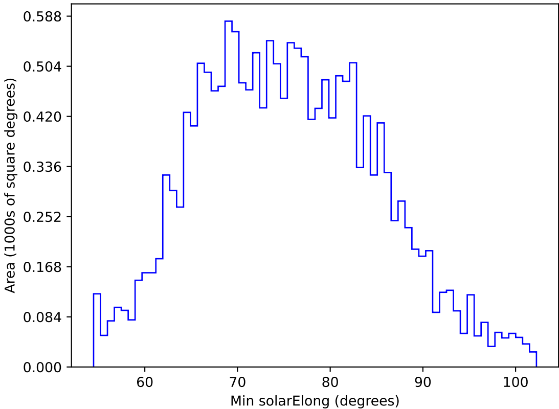
too_elab_r8_d3_ugrizy_v3.4_10yrs WFD u band: Min solarElong
