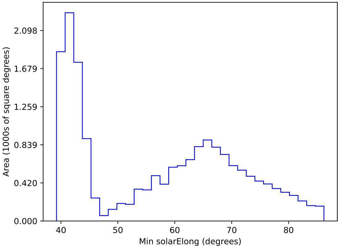
too_elab_r8_d3_ugrizy_v3.4_10yrs WFD r band: Min solarElong
