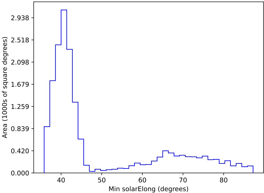
too_elab_r8_d3_ugrizy_v3.4_10yrs WFD i band: Min solarElong
