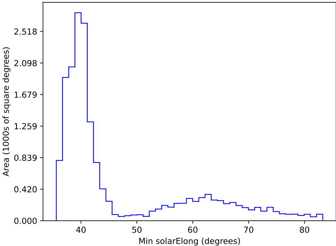
too_elab_r8_d3_ugrizy_v3.4_10yrs WFD all bands: Min solarElong
