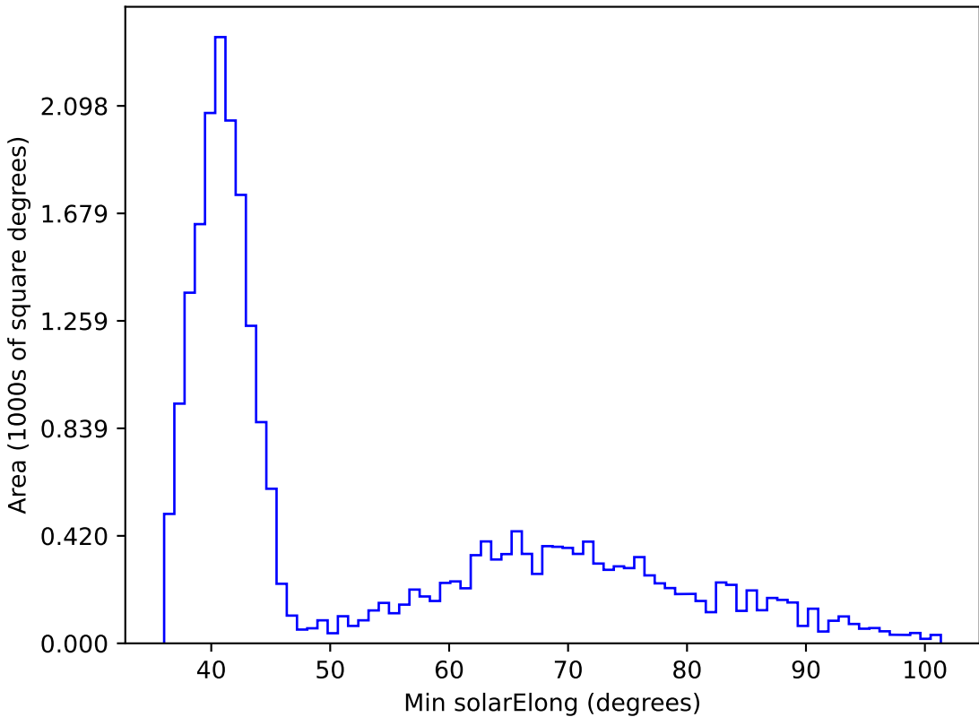
too_elab_r8_d3_ugrizy_v3.4_10yrs All sky z band: Min solarElong
