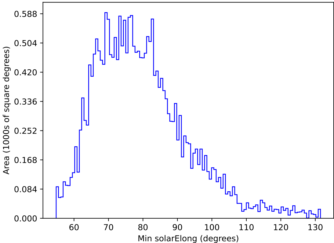
too_elab_r8_d3_ugrizy_v3.4_10yrs All sky u band: Min solarElong
