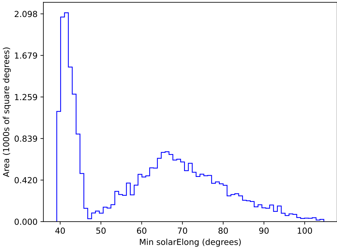
too_elab_r8_d3_ugrizy_v3.4_10yrs All sky r band: Min solarElong
