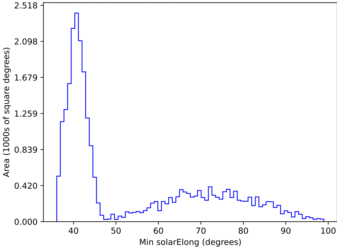
too_elab_r8_d3_ugrizy_v3.4_10yrs All sky i band: Min solarElong
