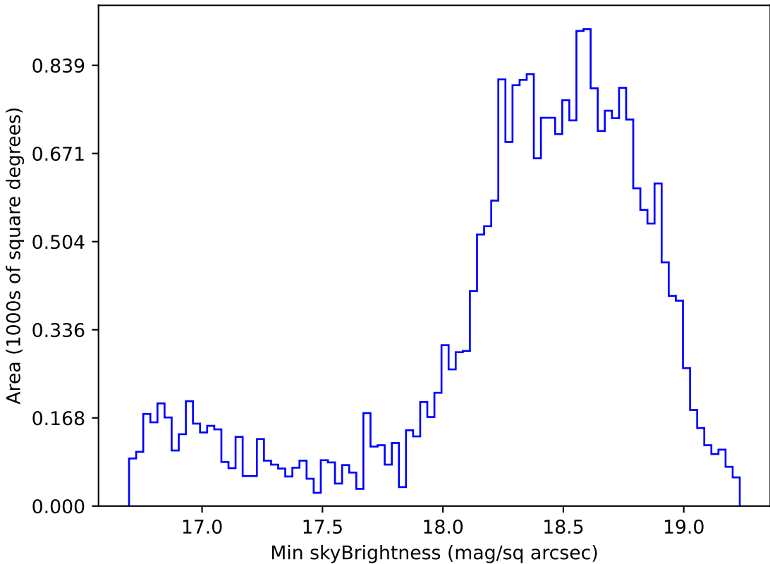
too_elab_r8_d3_ugrizy_v3.4_10yrs Yr 1 z band: Min skyBrightness
