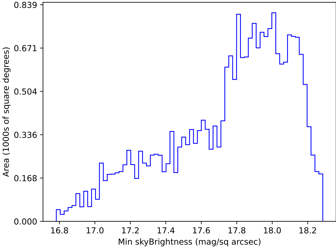
too_elab_r8_d3_ugrizy_v3.4_10yrs Yr 1 y band: Min skyBrightness
