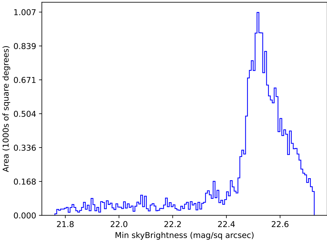
too_elab_r8_d3_ugrizy_v3.4_10yrs Yr 1 u band: Min skyBrightness
