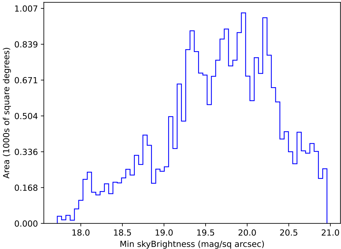
too_elab_r8_d3_ugrizy_v3.4_10yrs Yr 1 r band: Min skyBrightness
