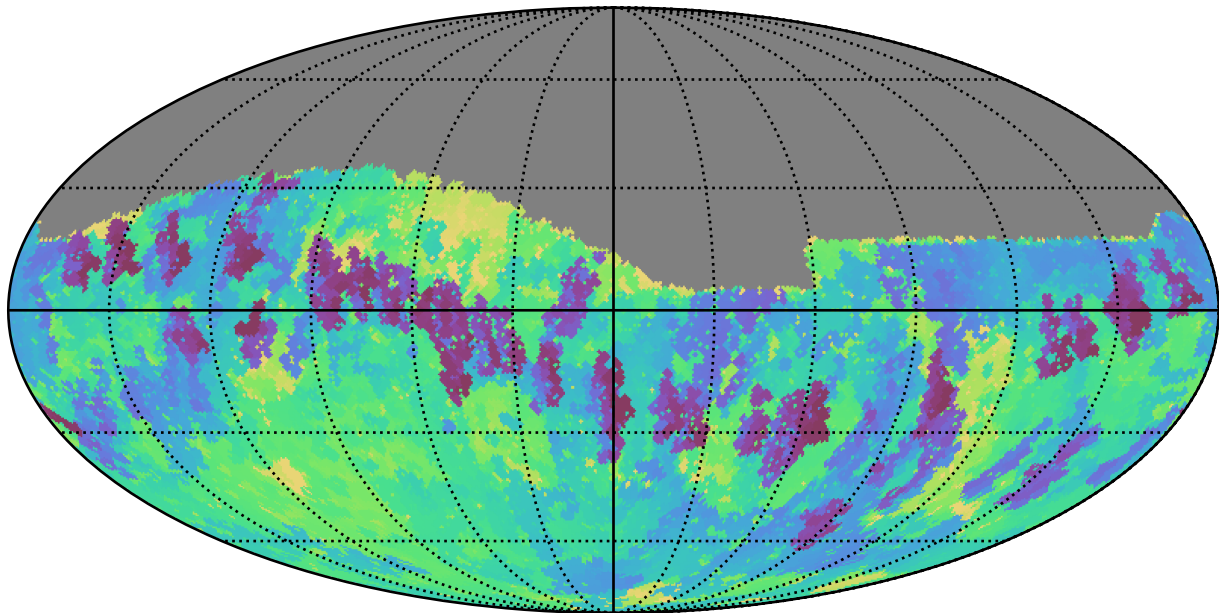
too_elab_r8_d3_ugrizy_v3.4_10yrs Yr 1 i band: Min skyBrightness
