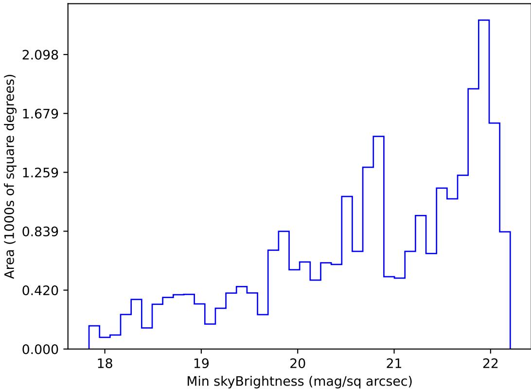
too_elab_r8_d3_ugrizy_v3.4_10yrs Yr 1 g band: Min skyBrightness
